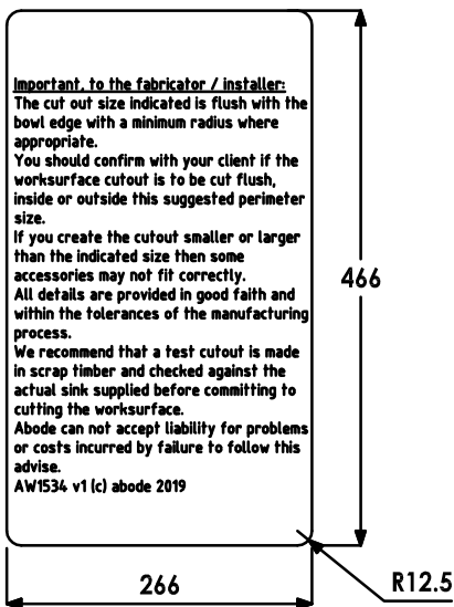
UNDERMOUNT CUT OUT
