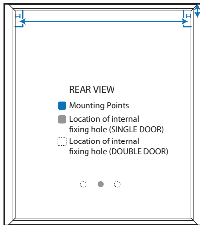
Fixing Preparation (Fig A)
