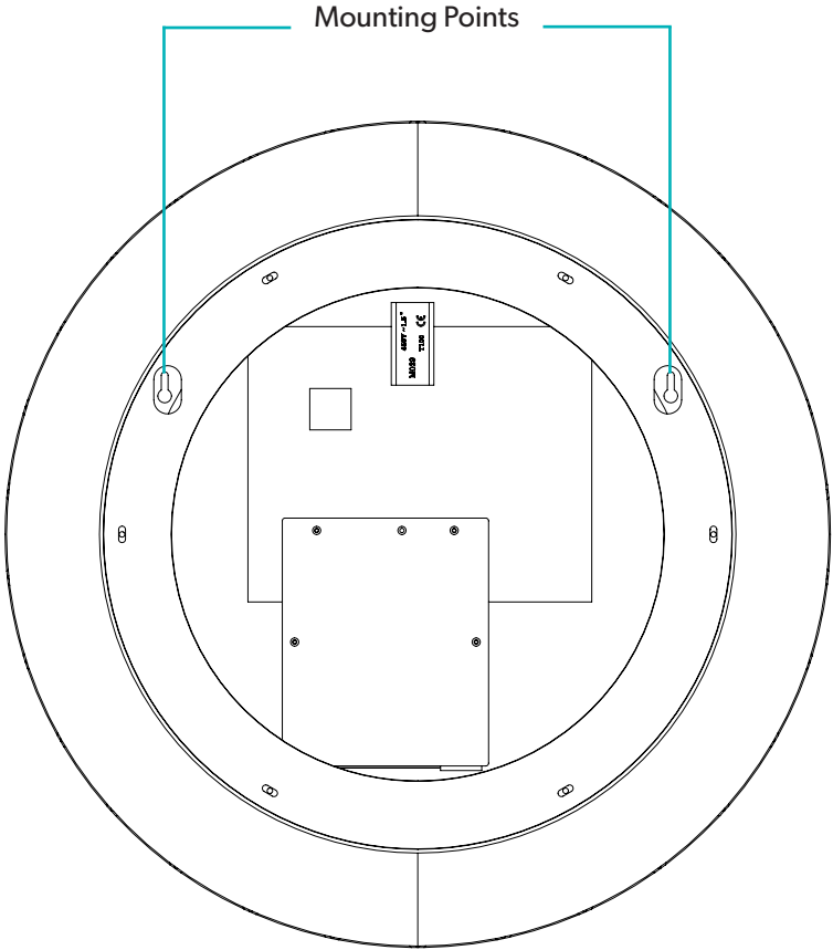
Fig 2. - Mounting points
